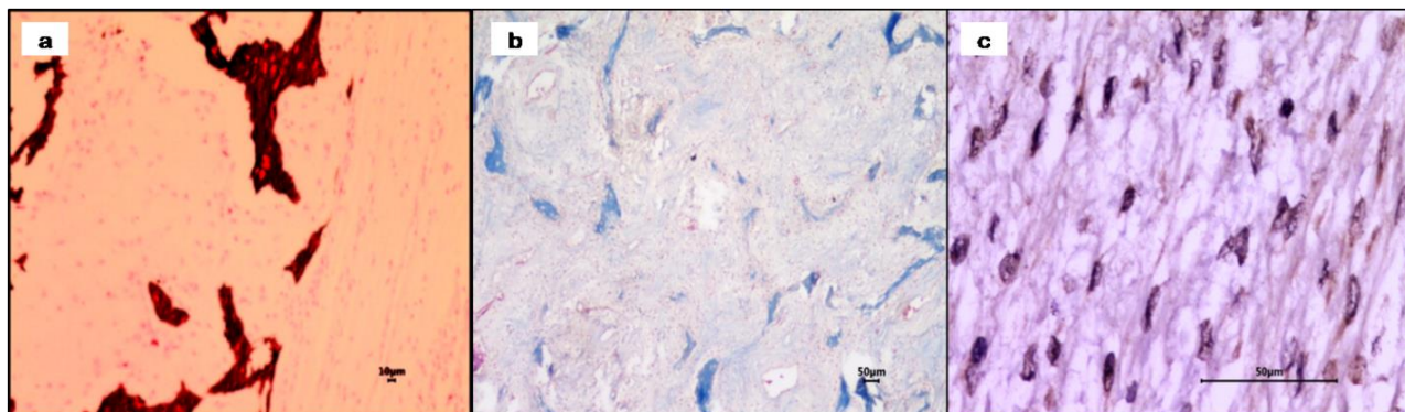
Fig. 6: Undecalcified sections of the mandible. (a) Von Kossa stain demonstrating sparsely distributed black stained calcified bone trabeculae (von Kossa stain, ×100), (b) Masson's trichrome stain showing extensive deposition of collagen fibers (blue) of various levels of maturation and immature osteoid (Masson's trichrome stain, ×40), and (c) Fibroblasts showing strong nuclear PCNA immunostaining (DAB, ×400)
