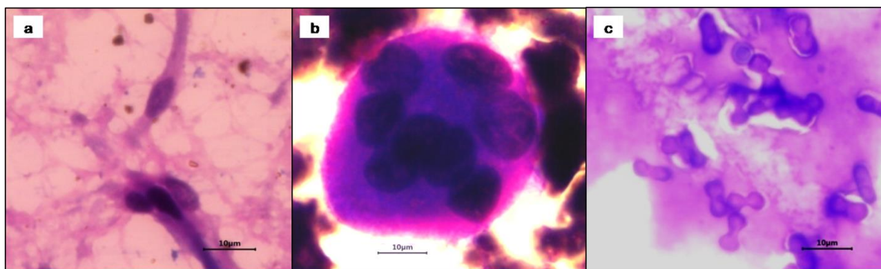
Fig. 3: Microscopic evaluation of fine needle aspiration cytology of the mandible (Giemsa stain, \times 1000 ). Scanty cellular smears with abundant proteinaceous background material, (a) Clusters of fibroblasts, (b) Individual multinucleated osteoclast, and (c) Aggregates of binucleated chondrocytes
