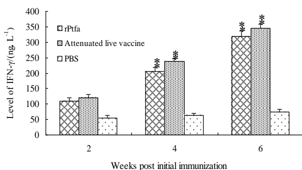
Fig. 4: The level of IFN- \gamma secreted by peripheral blood lymphocytes from immunized chickens. ConA was added to stimulate peripheral blood lymphocytes 2, 4 and 6 weeks after the first immunization. ** P<0.01
