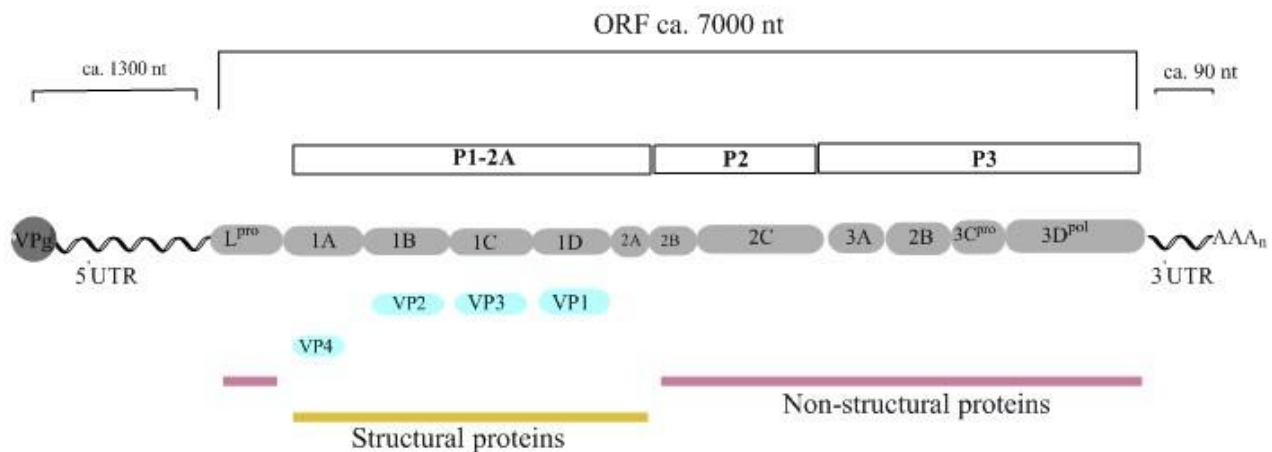
Fig. 1: The FMDV RNA genome contains a single large open reading frame (ca. 7000 nt), which encodes a large polyprotein being processed into primary products: L^{pro} , P1-2A, P2, and P3 in a protease independent break. Cleavage of P1-2A by the 3C protease ( 3C^{pro} ) is essential for producing four capsid proteins (VP1-VP4) and 2A. P2 and P3 regions produce non-structural proteins: 2B, 2C, 3A, 3B1-3, or Vpg, 3C^{pro} , 3D^{pol} that are involved in virus replication and pathogenesis. The each side of the genome is included in a large 5' UTR region (ca. 1300 nt) and a small 3' UTR (ca. 90 nt), ending in a poly-A tail
