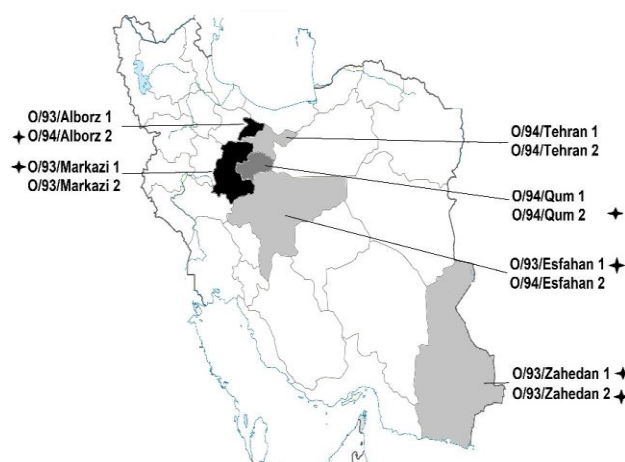
Fig. 2: The distribution of samples received from the foot-and-mouth disease outbreak area during 2015-2016. The name of samples related to each province are displayed. \blackrightarrow Indicate samples that used in antigenic relationship evaluation by 2D-VNT test
